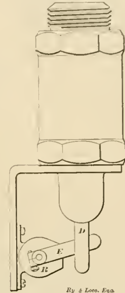
AIR PUMP STROKE COUNTER.
